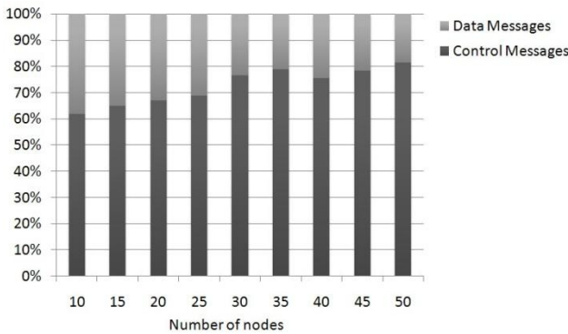
Fig. 5. Overhead ratio according to different number of nodes
