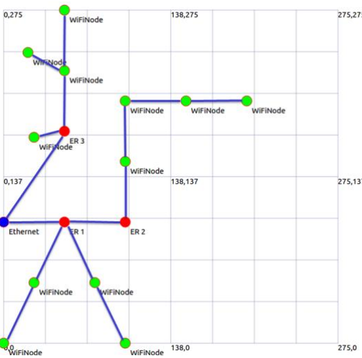
Fig. 3. Sample hybrid network and DODAG building
