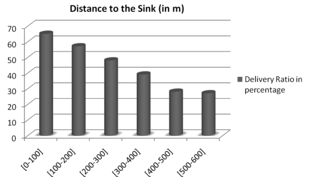
Fig. 4. Delivery ratio versus distance to the sink (or edge router)
