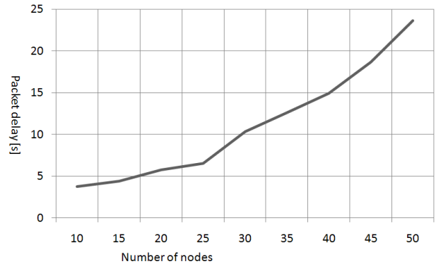
Fig. 7. Packet delay with varying node density
