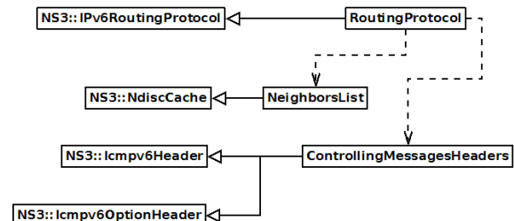
Fig. 1. Simplified class diagram of module
